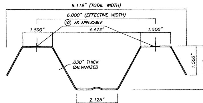
1A HALF PANEL
