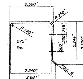
4 "U" HEADER
