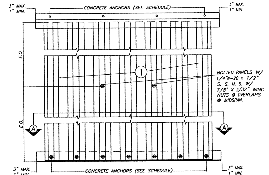
STORM PANEL TYPICAL ELEVATION
