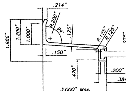
5 3" ANGLE BUILD OUT BRACKET
