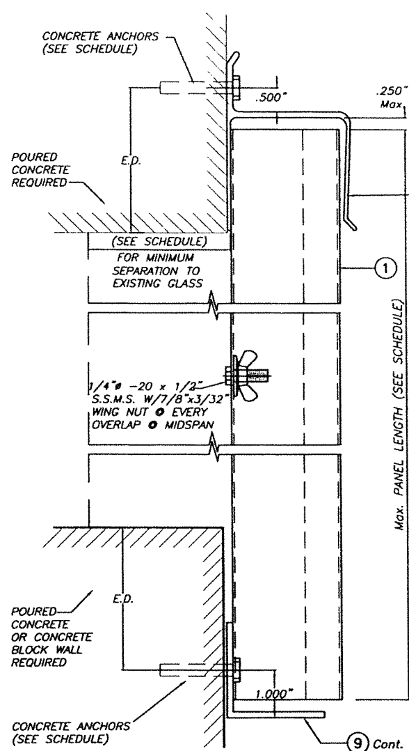
SECTION 1 ANCHOR
