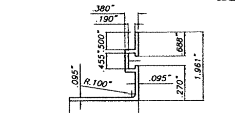
7 REVERSED "F" ANGLE TRACK
