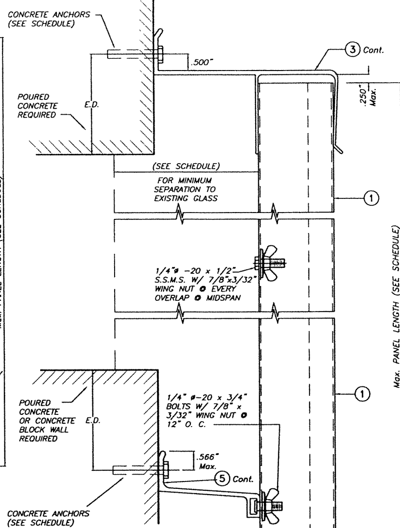
BUILD OUT INSTALLATION SECTION 3 SCALE : 3/8" = 1"
