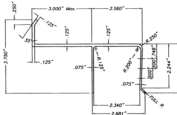
3 3" Max. "U" BUILD OUT
