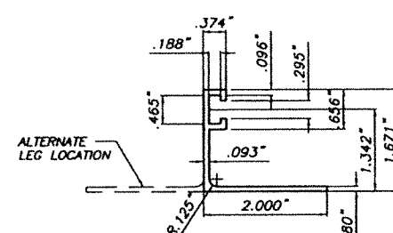
8 "F" TRACK ANGLE
