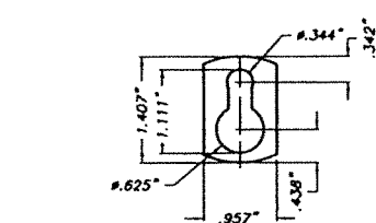
11 KEY HOLE WASHER
