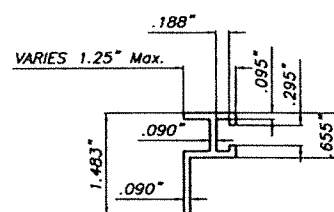
6 "F" TRACK
