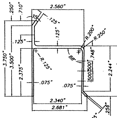
2 "h" HEADER
