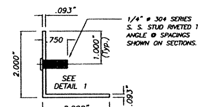
9 STUDDED ANGLE
